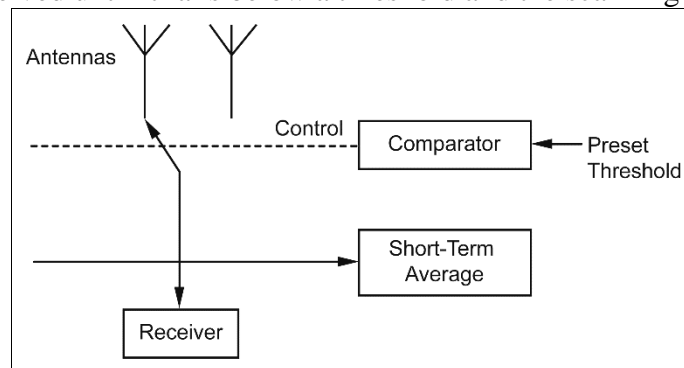
Fig. 4.48. Block diagram of feedback diversity
