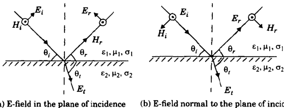
Figure 1.2: Geometry for calculating the reflection coefficients between two dielectrics
