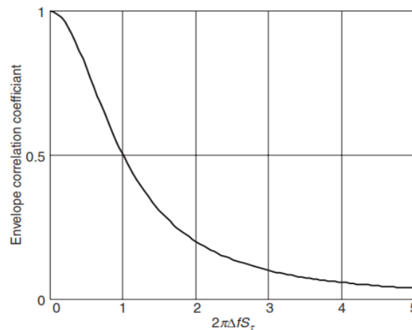
Fig. 4.13. Correlation coefficient of the envelope as a function of normalized frequency spacing.
