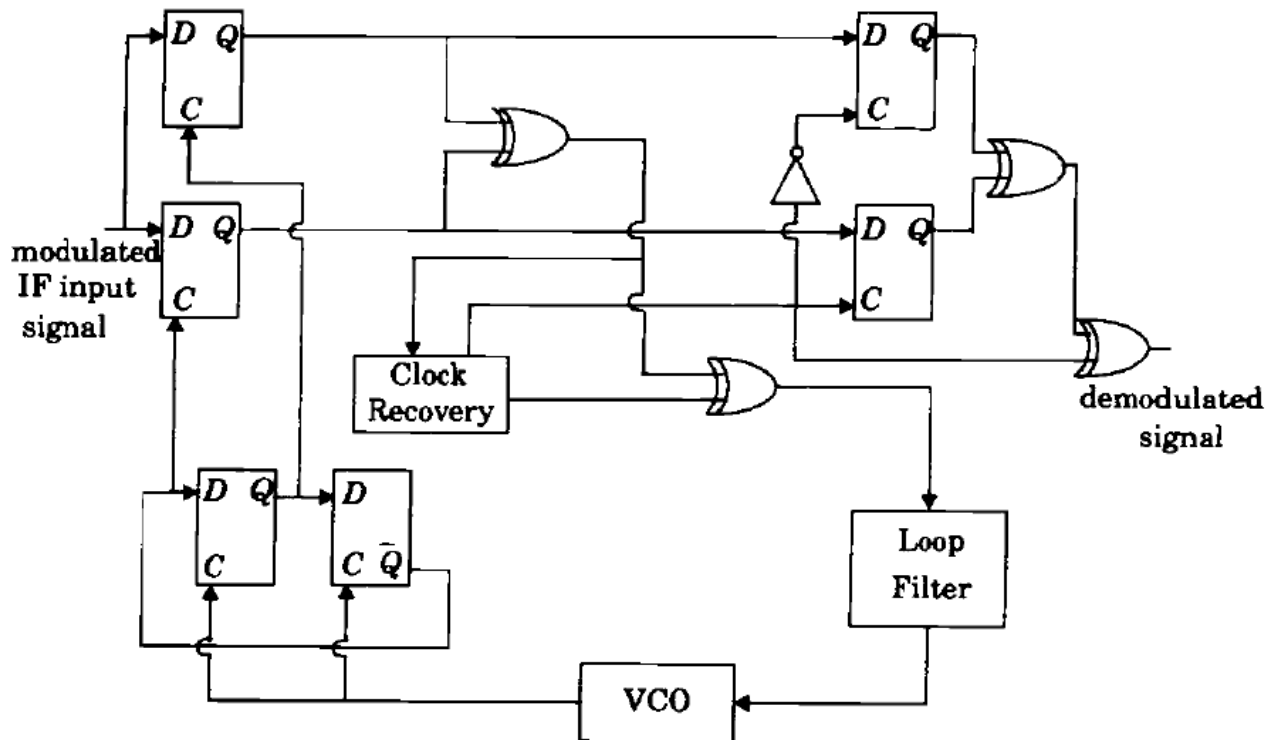
Figure: Digital logic circuit for GMSK demodulation
