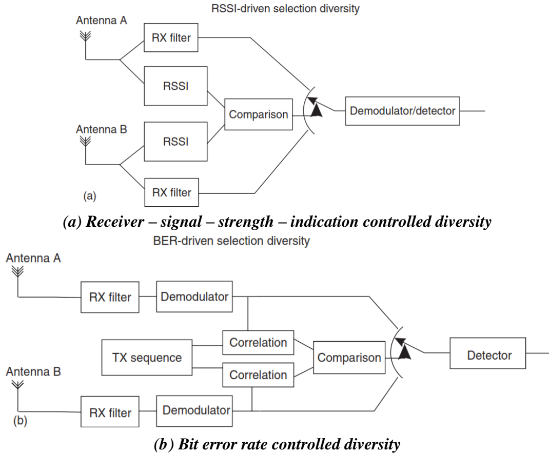
Fig. 4.37. Selection diversity principle
