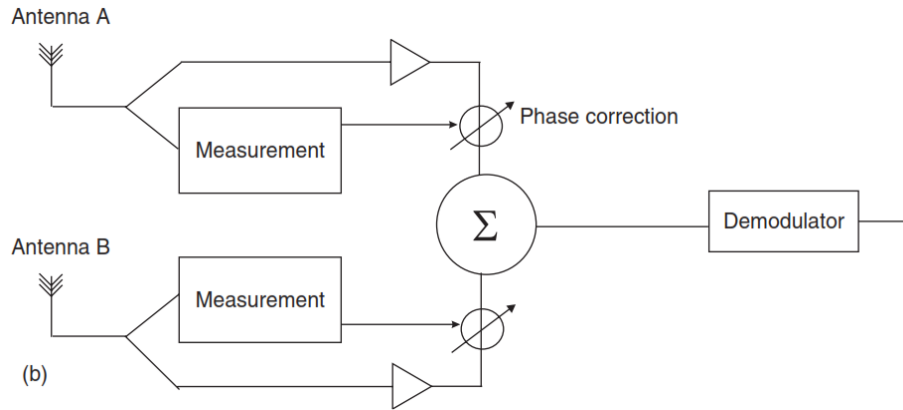
(b) Equal gain combining
