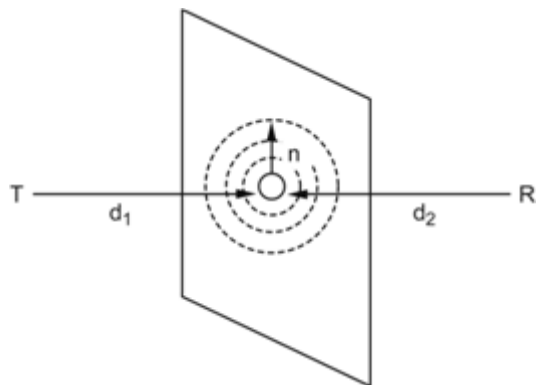
Figure 1.7: Fresnel zones
