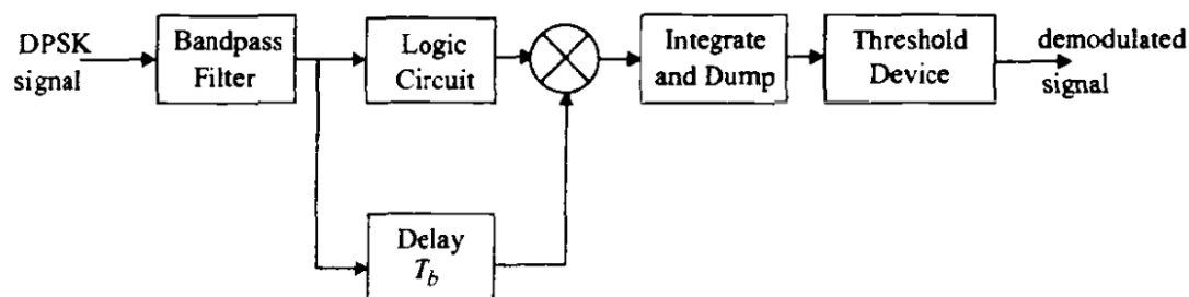
Figure. Block diagram of DPSK receiver.
