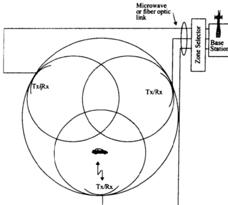
Figure: The microcell concept
