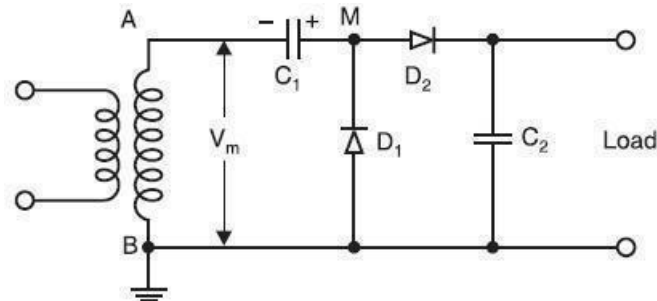
Figure:3.2 Greinacher voltage doubler circuit
