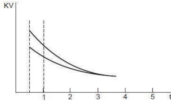
Figure:5.1 Voltage-time curve of typical major insulation in transformer
