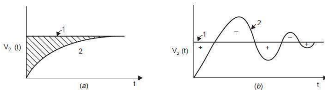
Figure:4.15theresponseofresistancevoltage divider
