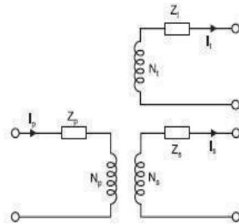
Figure:3.9Equivalent circuit of a three-winding transformer
