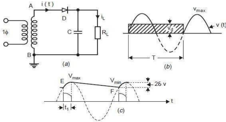
Figure: 3.1 (a) Single Phase rectifier (b) Output voltage without C (c) Output voltage with C If the circuit is loaded, the output voltage does not remain constant at V_{\max} . After point E (Fig. 3.1 (c)), the supply voltage becomes less than the capacitor voltage, diode stops conducting.
