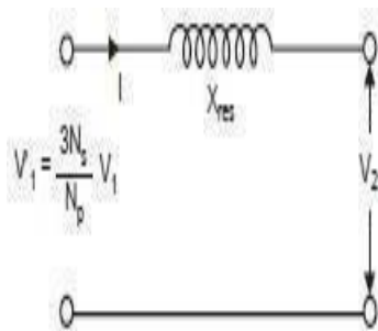
Figure:3.10Equivalentcircuitof3-stagetransformer
