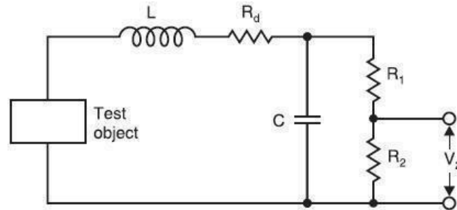
Figure:4.14Simplifieddiagramofaresistancepotentialdivider
