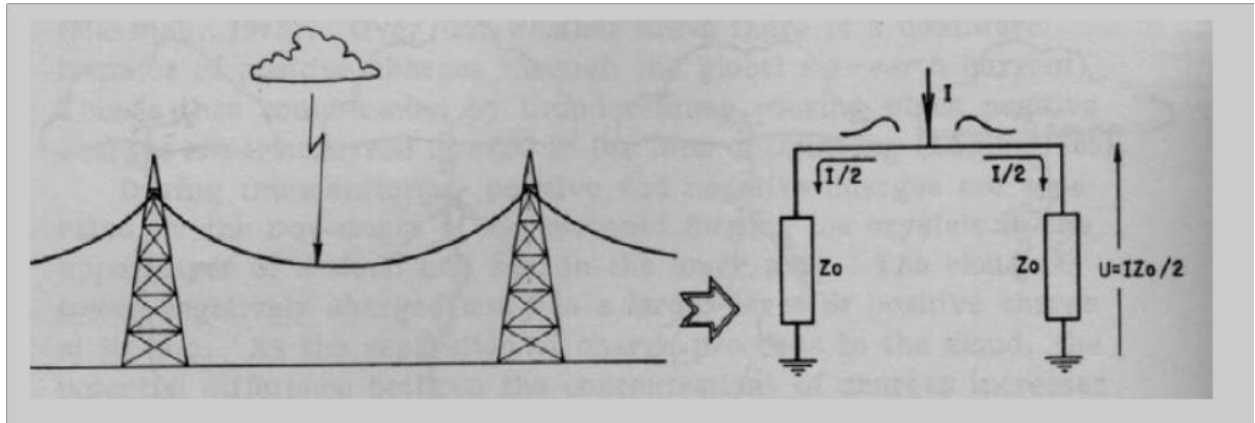
Figure:1.3 Developmental Lightning overvoltage
