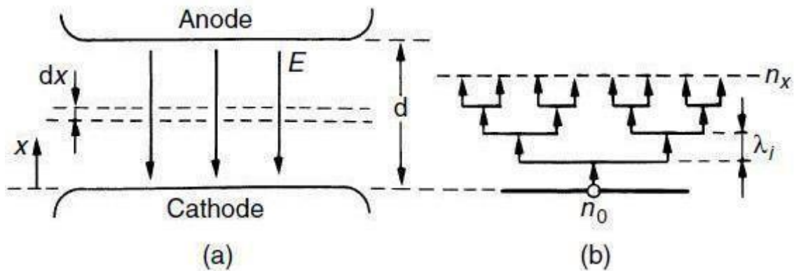
Figure:2.5 Schematic representation of electron multiplication (a) gap arrangement, (b) Electron avalanche
