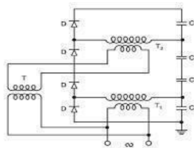
Figure:3.6Cascadedrectifiercircuit
