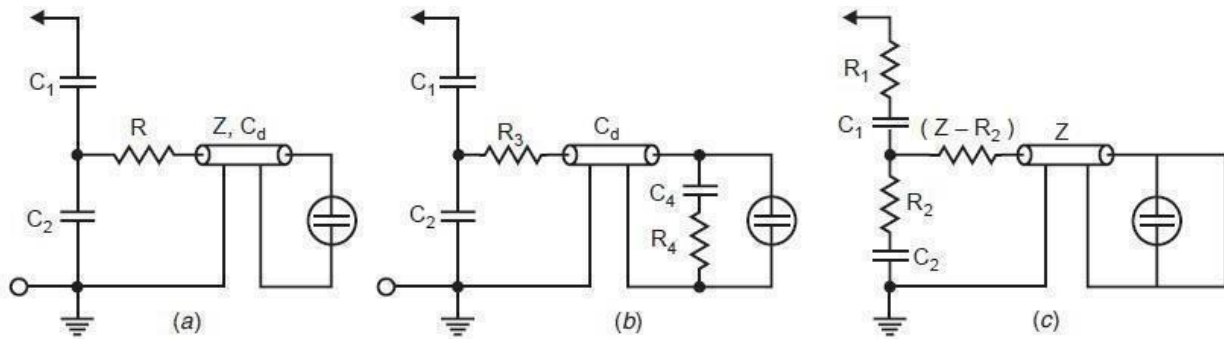
Figure: 4.13 Capacitor dividers (a) Simple matching (b) Compensated matching (c) Damped capacitor dividers. For voltage dividers in FIG. (b) and (c), the delay cable cannot be matched at its end.
