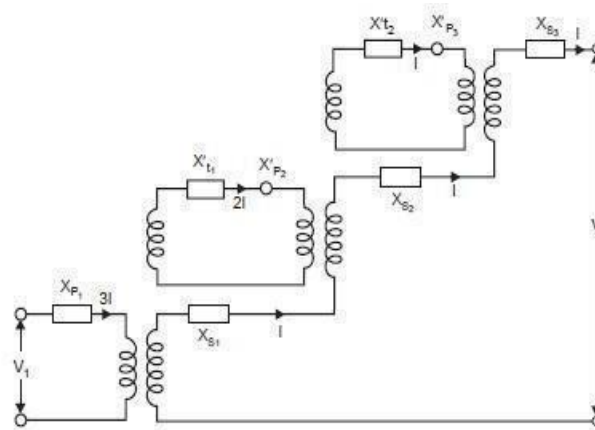
Figure:3.10Equivalentcircuitof3-stagetransformer
