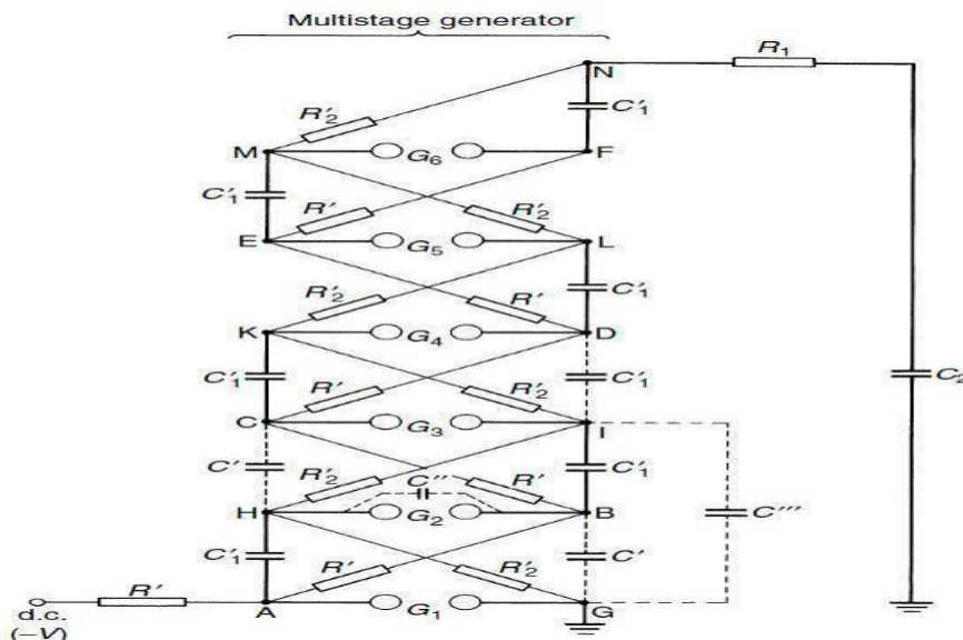
Figure:3.23Basiccircuitofasix-stageimpulsegenerator(Marxgenerator)resistances
