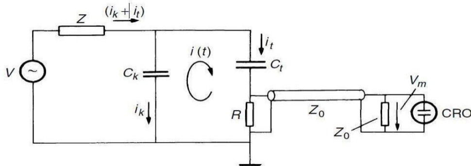
Figure:5.11 Measurement of PD current flow sensitivity circuit
