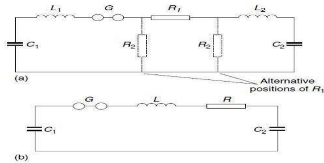
Figure:3.22Simplifiedcircuitofimpulsegeneratorandload.Circuits showing alternativepositionsofthewavetailcontrolresistance.(b)Circuitfor calculationof wave frontoscillations
