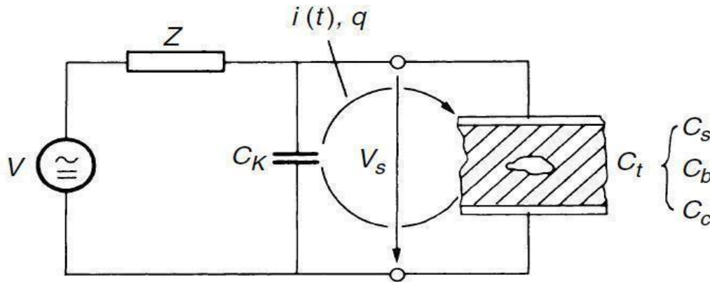
Figure:5.10The PDtestobject C_t within a PDtestcircuit
