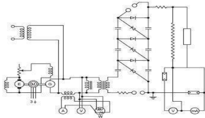
Figure:3.5ATypicalCockroftcircuit
