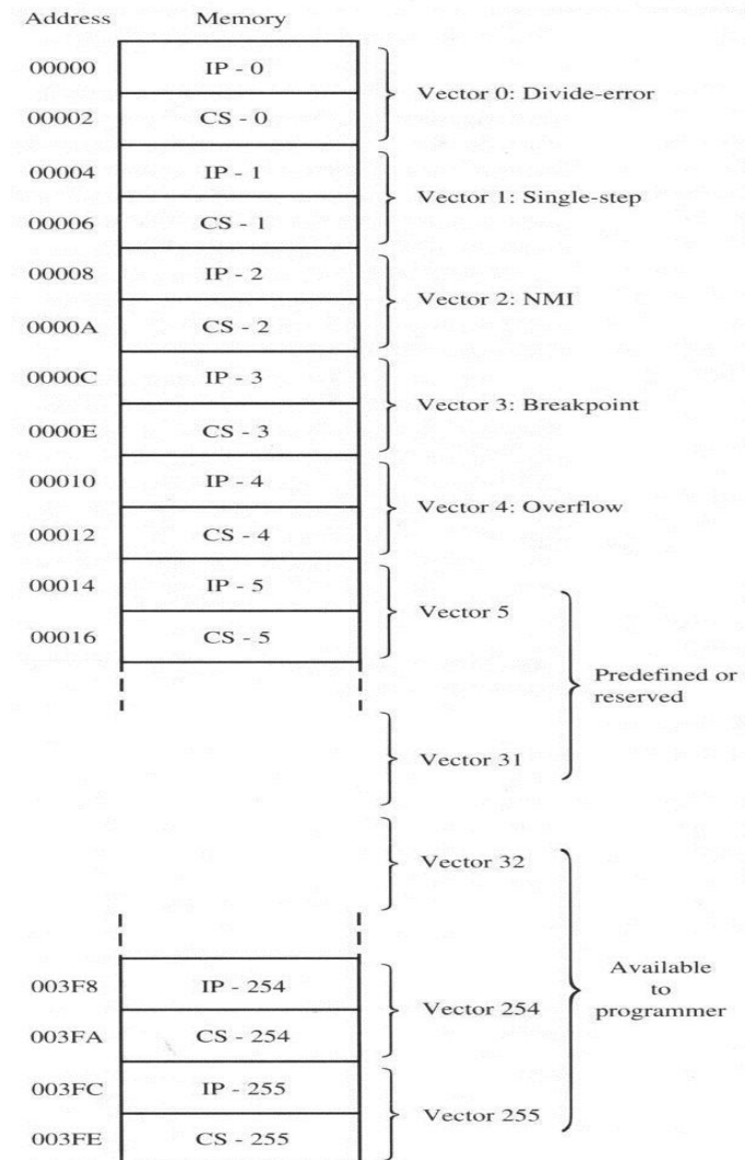
Figure 1.3 Organisation of Interrupt Vector Table in 8086
